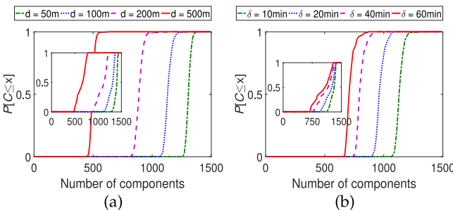
Fig. 11. Distribution of the number of components C when aggregating over all the samples of two days in Beijing trace: (a) The CDFs for different transmission distances d with the delay tolerance \delta = 10 min, and (b) the CDFs for different delay tolerance \delta with the transmission distance d = 100 m. The main plot is for the daytime, while the subplot inside is for the nighttime.
